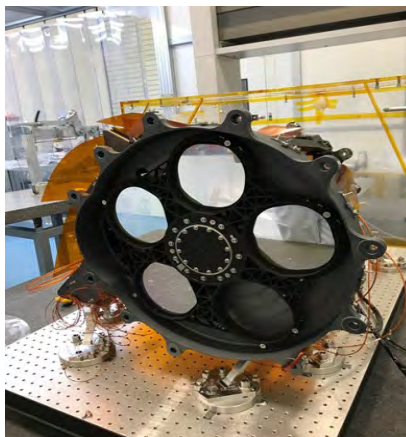
Grisms for NISP instrument (EUCLID Mission)
