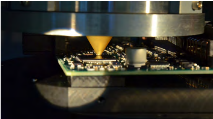
SQUID Sensor analysing the current track on assembled PCB (Magnetic microscopy)
